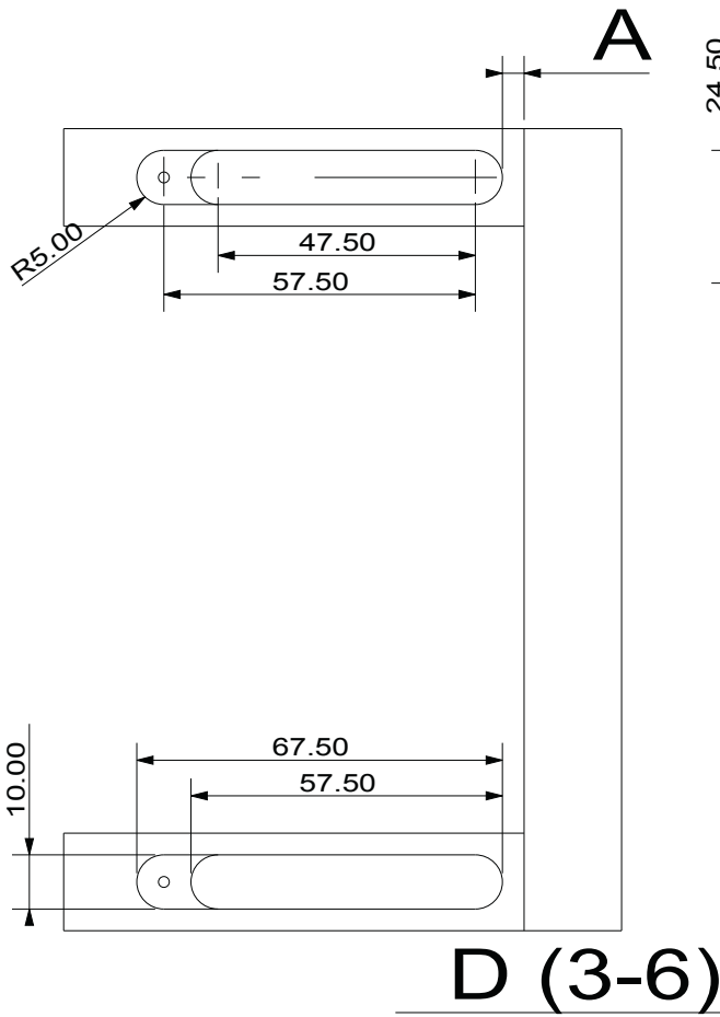
BASE/CAPPELLO BASE/HAT
